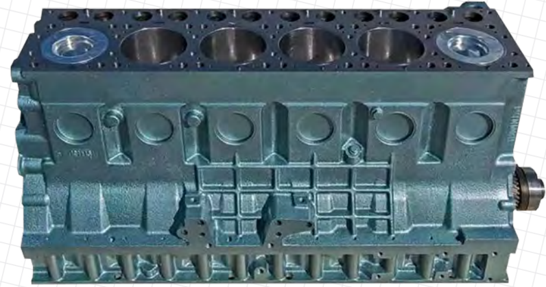
ENGINE BLOCK
