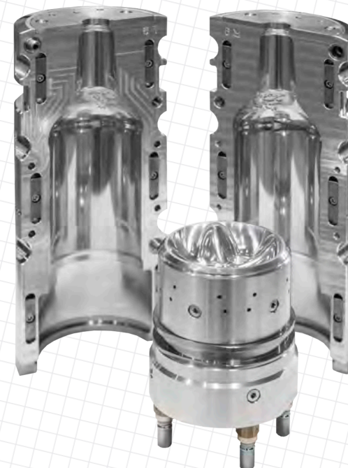
BLOW MOULD PISTONS
